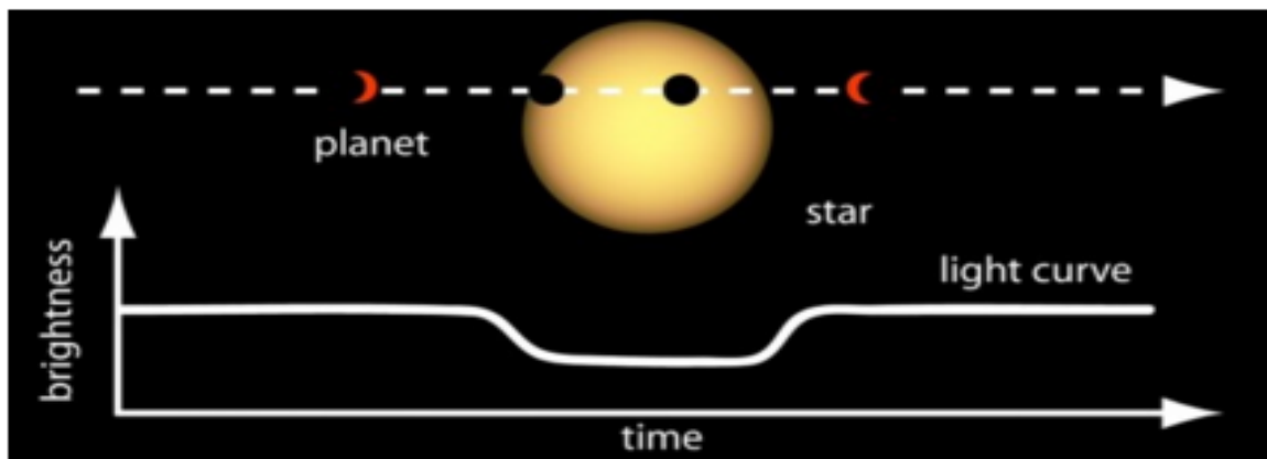
An illustration of planetary “transit” in front of its star
