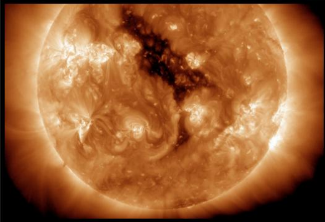
Solar wind flowing from the indicated coronal hole should reach Earth on April 4-5. Credit: SOO/JAXA.
