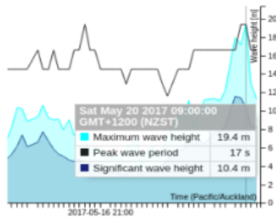
Chart showing the measurements of the largest wave ever measured in the Southern Ocean by a buoy on May 20, 2017 via MetOcean
