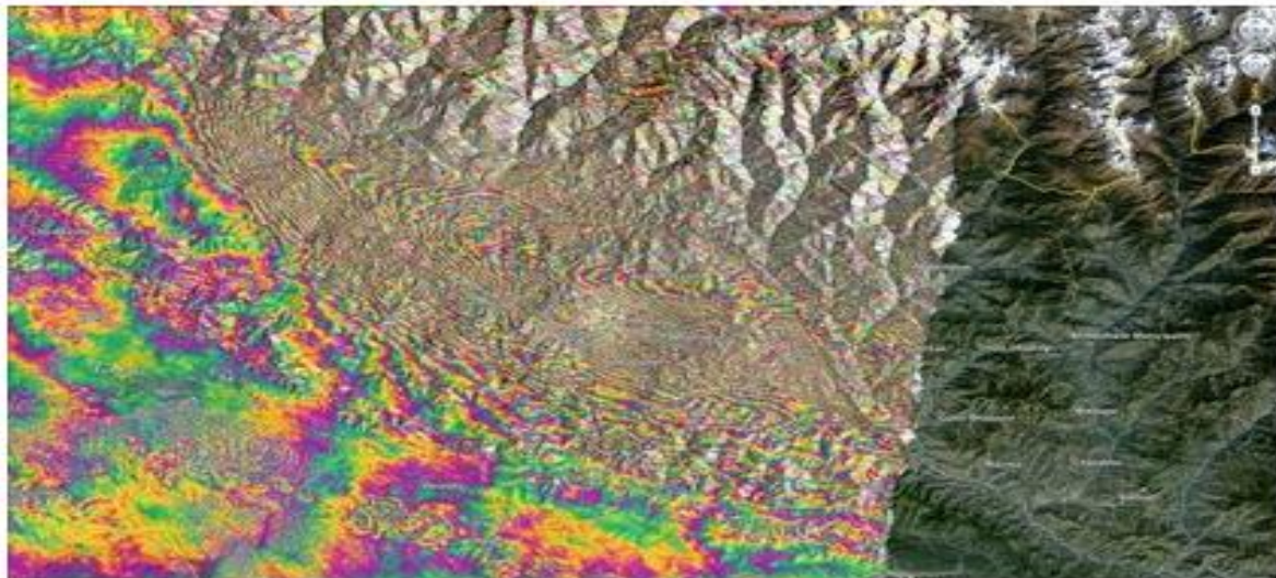
Satellite radar image of the ground changes due to the magnitude-7.8 Nepal earthquake on April 25.
