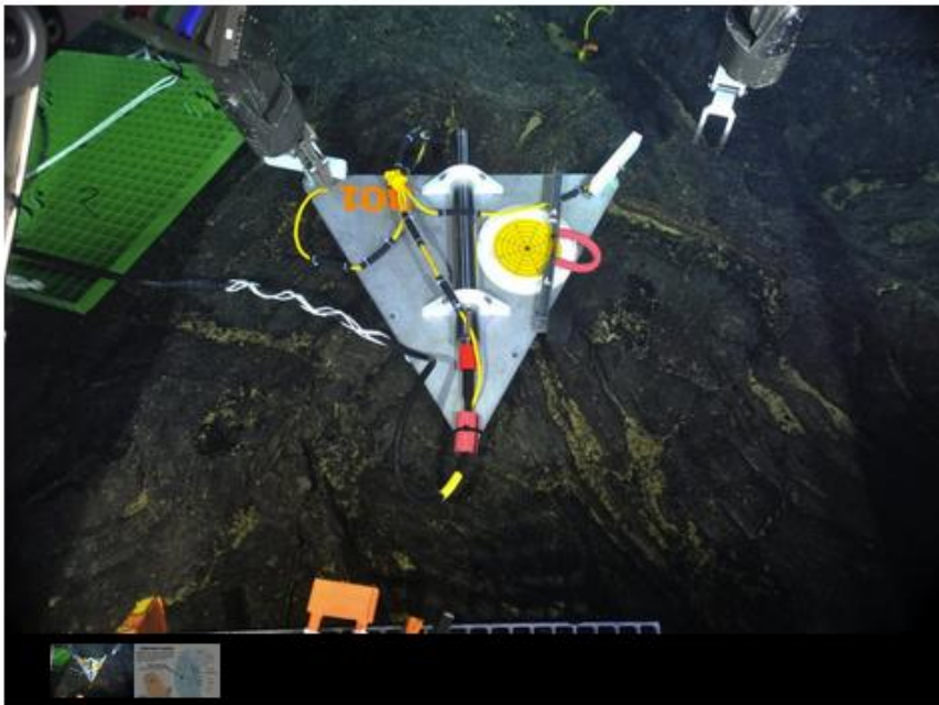
1 of 2 A seismometer is deployed on the underwater Axial Volcano in 2014. (National Science Foundation's Ocean Observatories Initiative / University of Washington... More ▾
