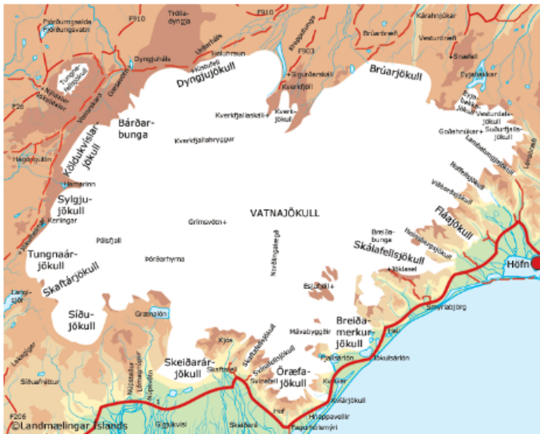
The largest glacier of Iceland Vatnajökull and the volcanoes buried under its ice.
