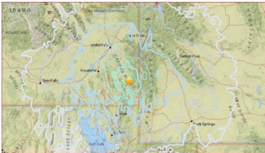
A M5.3 earthquake rocked Idaho on September 2, 2017 with tremors felt 200 miles away.
