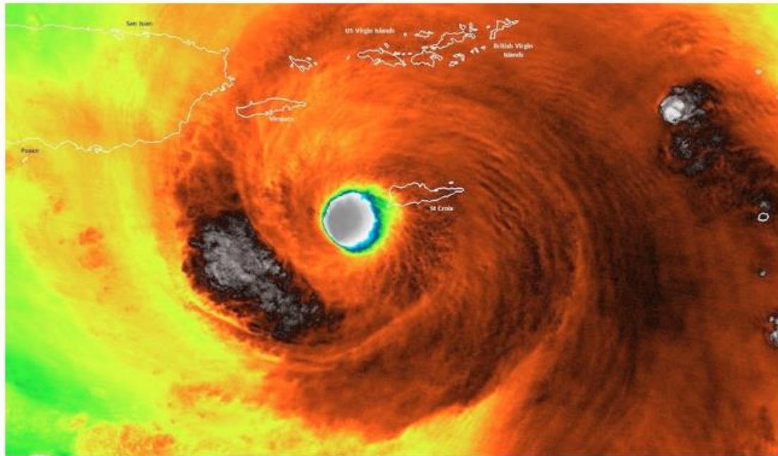
Above: VIIRS infrared satellite image of Hurricane Maria moving just west of St. Croix while at Cat 5 strength at 2:13 am EDT Wednesday, September 20, 2017. Image credit: NOAA/CIMMS/UM-Madison .
