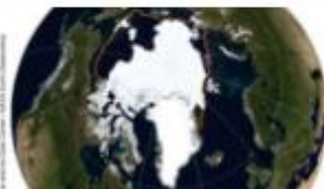
Arctic sea ice as of September 10, compared to average between 1981-
