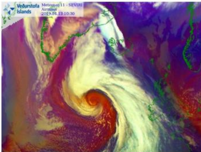
A spectacular deep 955 mbar 'bomb cyclone' is rapidly developing over the N Atlantic today. via Vedur.is
