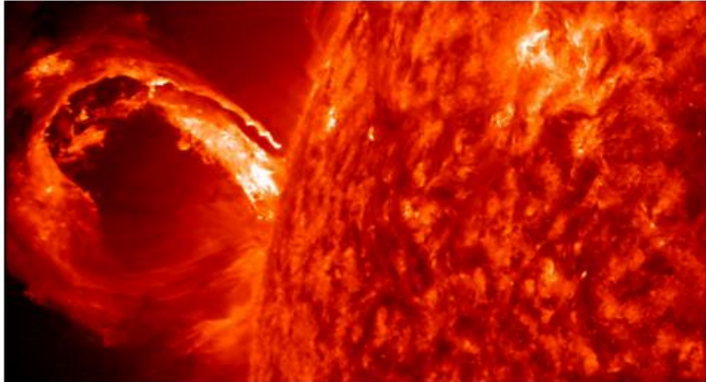
Powerful eruption from the surface of the sun captured on May 1, 2013. (NASA)
