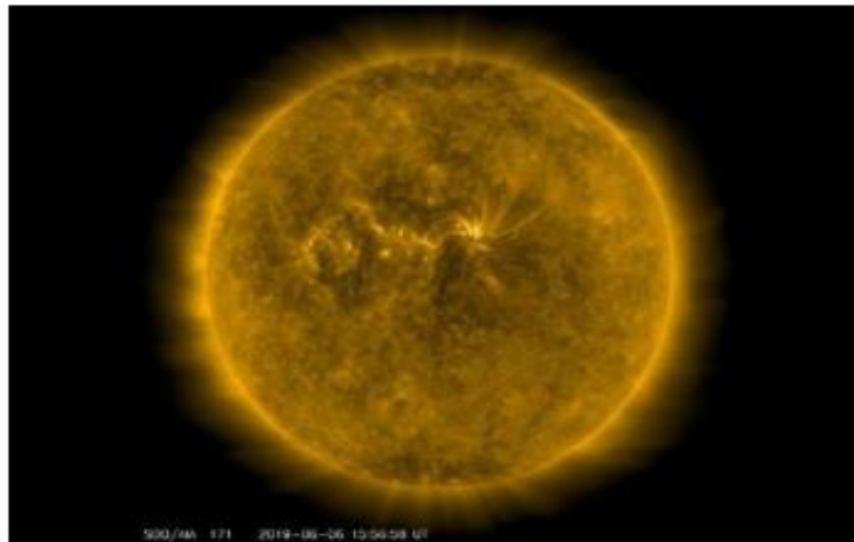
Spotless Surface Of The Sun Suggests We May Be Reaching The Solar Minimum. Photo: NASA/SDO
