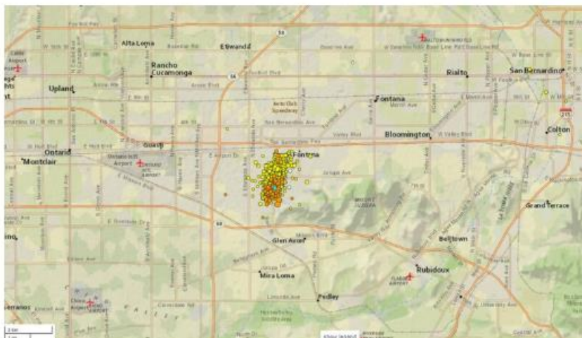
A flurry of small earthquakes in Fontana is taking an unexpected turn. (Orange dots represent quakes in the past week; yellow dots, quakes Friday.) (U.S. Geological Survey)
