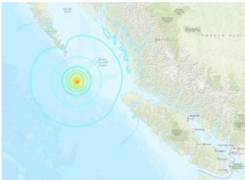
M6.2 earthquake lies off Vancouver Island, BC, Canada at the upper part of the Cascadia Subduction Zone On July 4, 2019. Earthquake map via USGS
