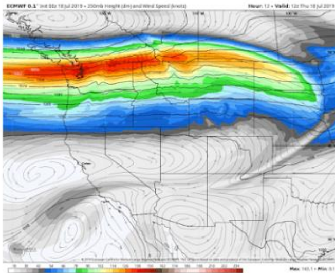
The strongest summer jet stream ever observed over the Pacific Northwest measured on July 18, 2019.
