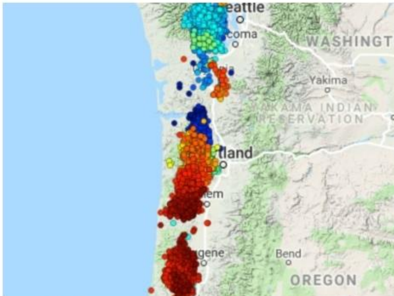
A map of ETS tremors from May, several months before the slow slip event began in Puget Sound. Map via PNSN
