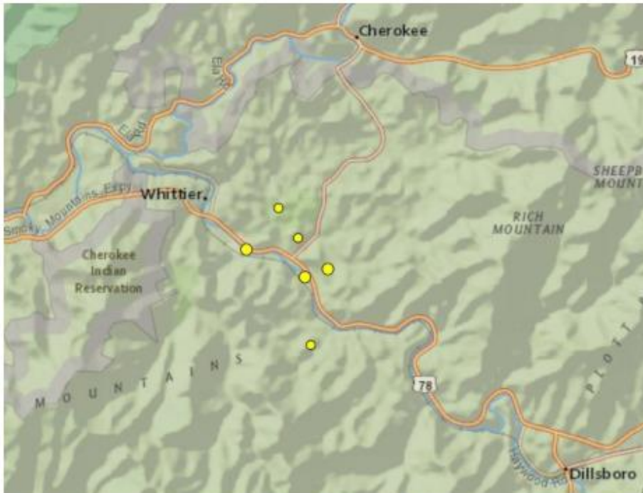
Six rare earthquakes rattle North Carolina in the last 5 days. Picture via USGS
