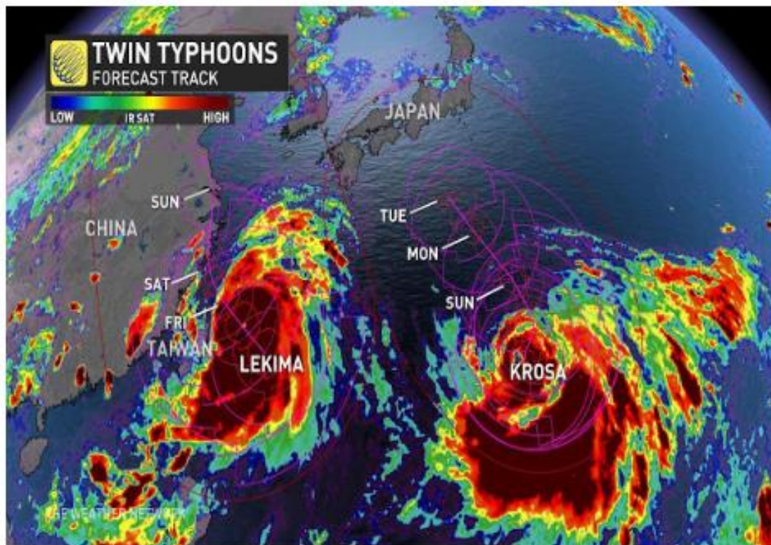
Photo, The Weather Network... Super typhoon Lekima followed by Tropical Storm Krosa
