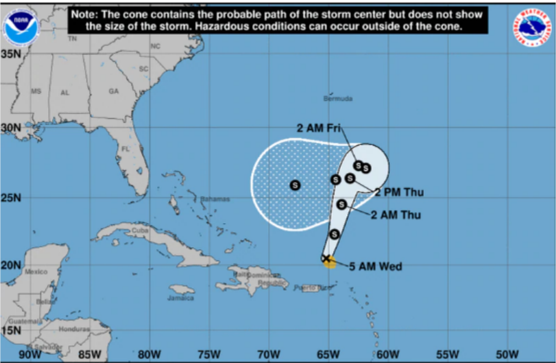
The cone of uncertainty for Tropical Storm Karen as of the National Hurricane Center's 5 a.m. Wednesday update. (The National Hurricane Center)
