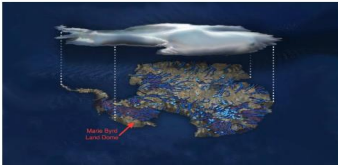
Map of flowing water under the Antarctic ice sheet. Blue dots indicate lakes, lines show rivers. Marie Byrd Land is part of the bulging "elbow" leading to the Antarctic Peninsula, left center. Credit: NSF/Zina Deretsky
