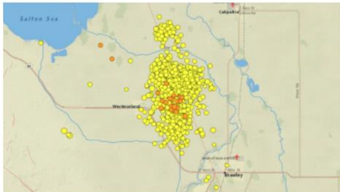
Earthquake Forecast for the Westmorland Swarm beginning September 30, 2020. Earthquake map via USGS
