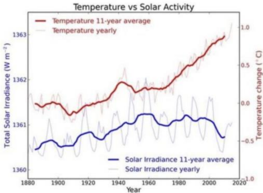
Global cooling over the next 20-30 years
