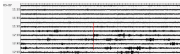
Strange seismograph signal after mysterious booms on Orcas Island, Washington State. Fig. Part of seismogram from station, ORCA on Mar 7, 2022. Note short strong signal (red) at 12:14:30 GMT (04:14:30 PST).
