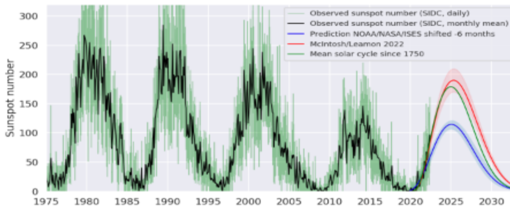
Sunspot numbers including predictions
